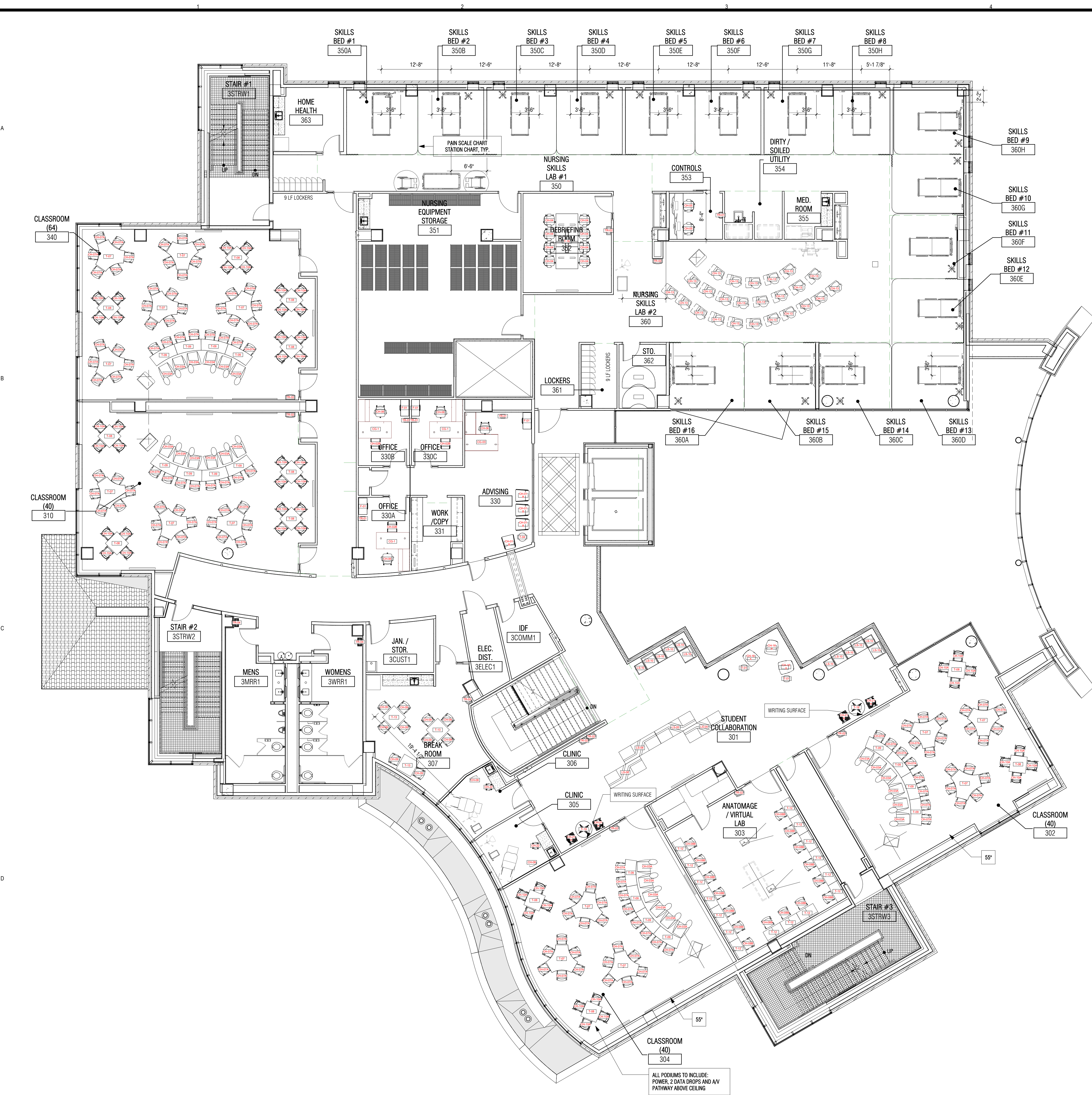
1 FURNITURE PLAN - LEVEL 3 1/8" = 1'-0"
